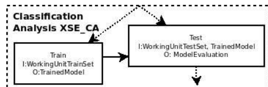
Figure 7. Classification Substructure
