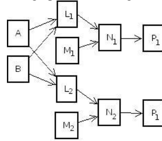
Figure 4. Graph after applying rules II. and III.
